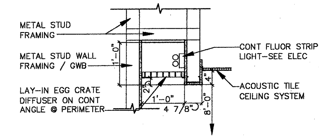
STANDARD RESTROOM LIGHT COVE DETAIL 3/4" = 1'-0"
