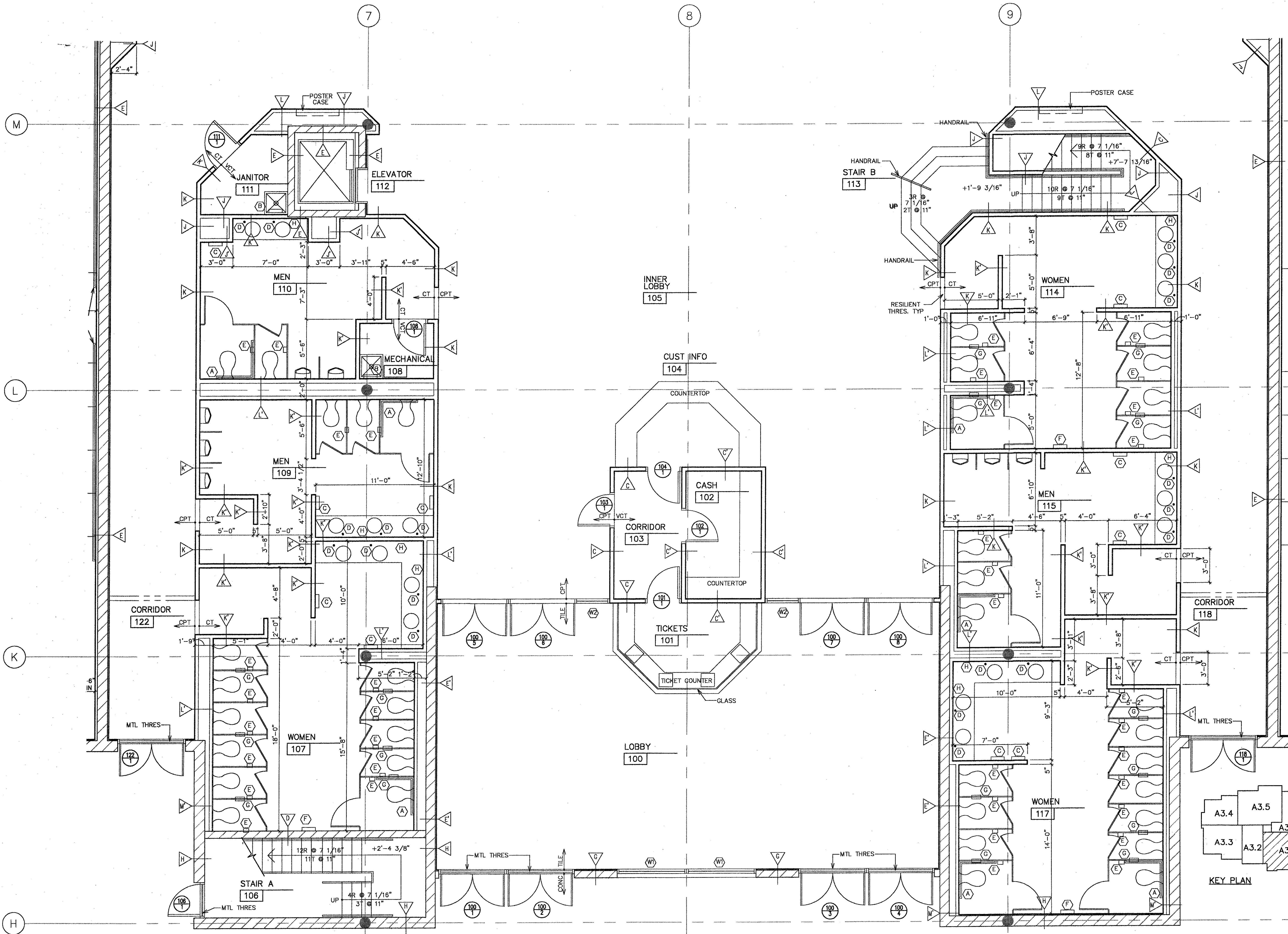
1 ENLARGED FLOOR PLAN-LOBBY CORE A3.1 1/4" = 1'-0"
