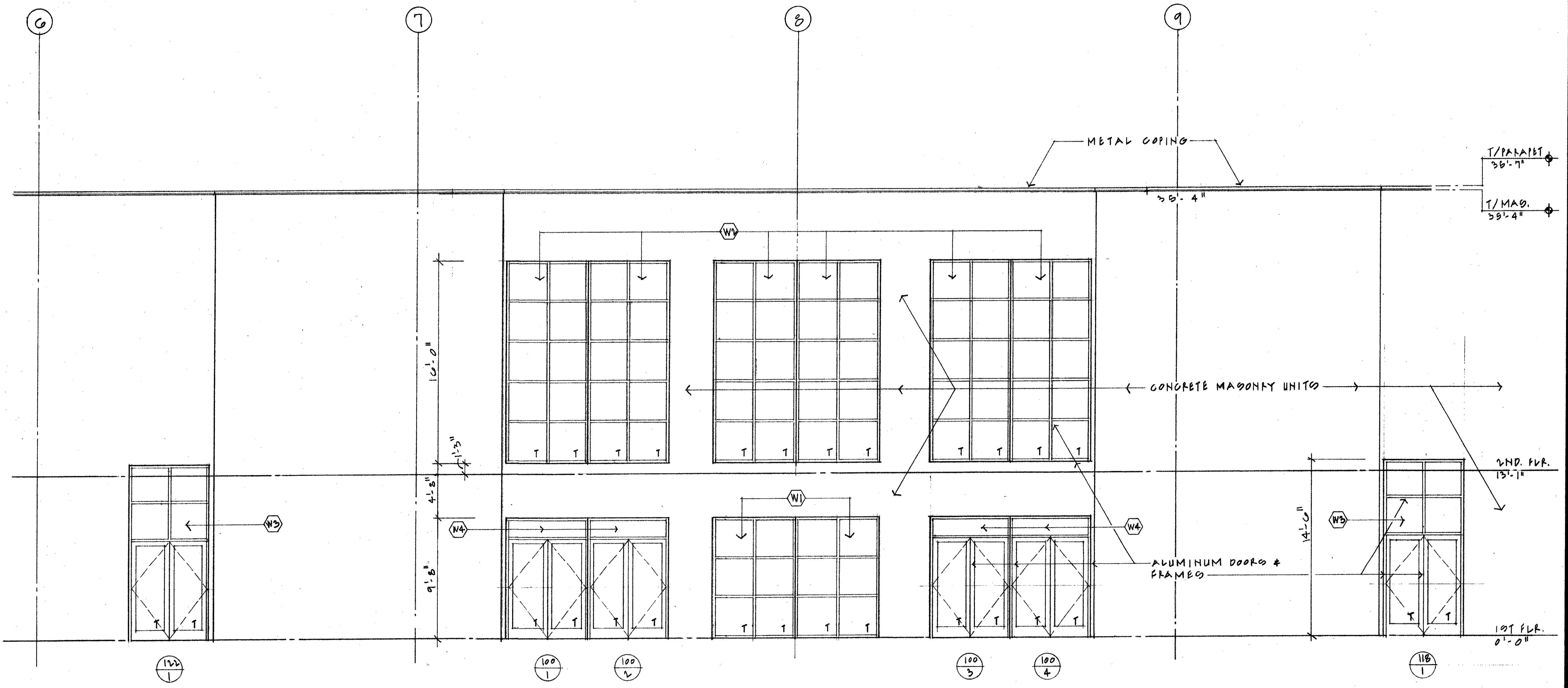
A PARTIAL ELEVATION - FRONT ENTRY 1/4" = 1'-0"
