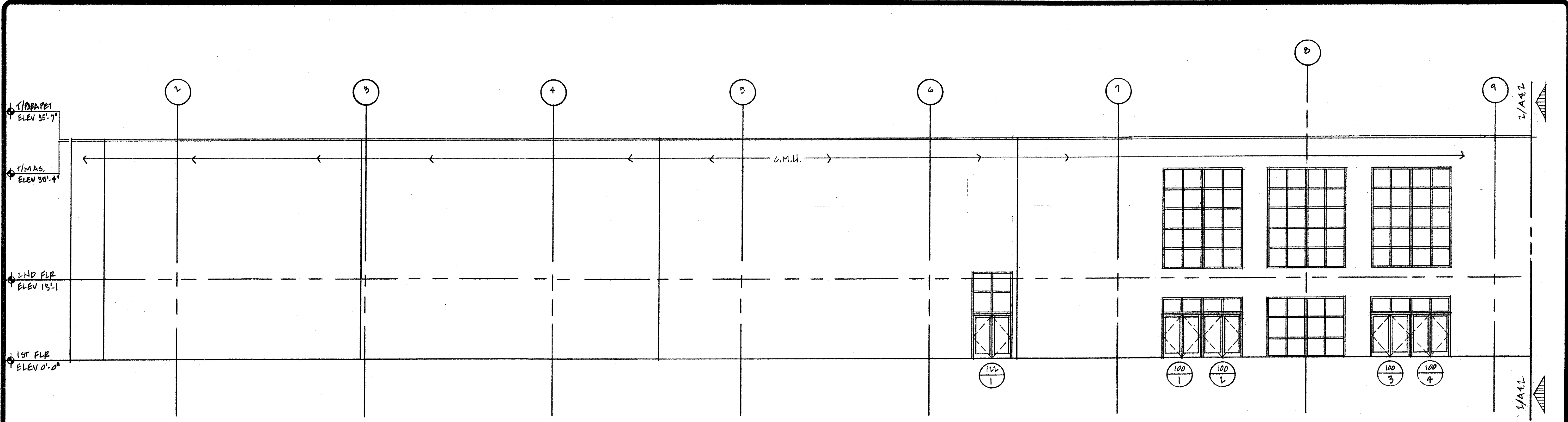
A BUILDING ELEVATION - NORTH (EAST QUADRANT) 1/8" = 1'-0"
