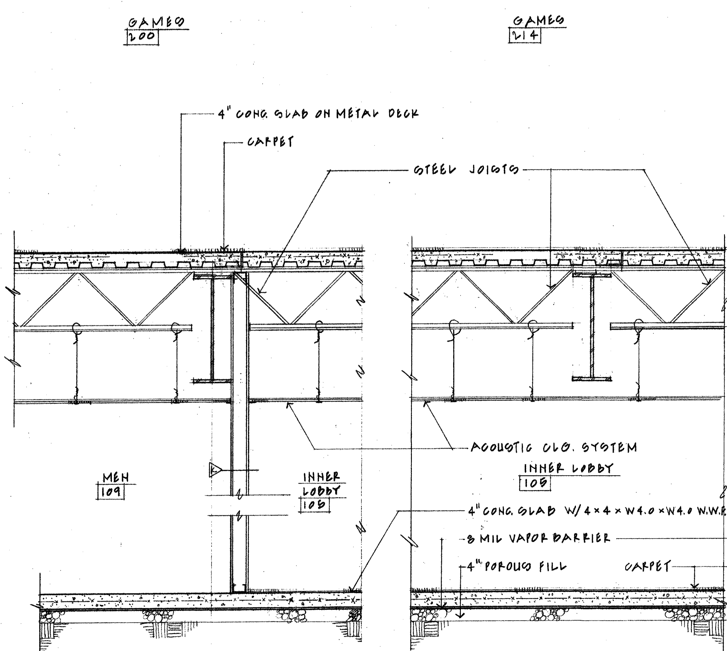
1 WALL SECTION 3/4" = 1'-0"
