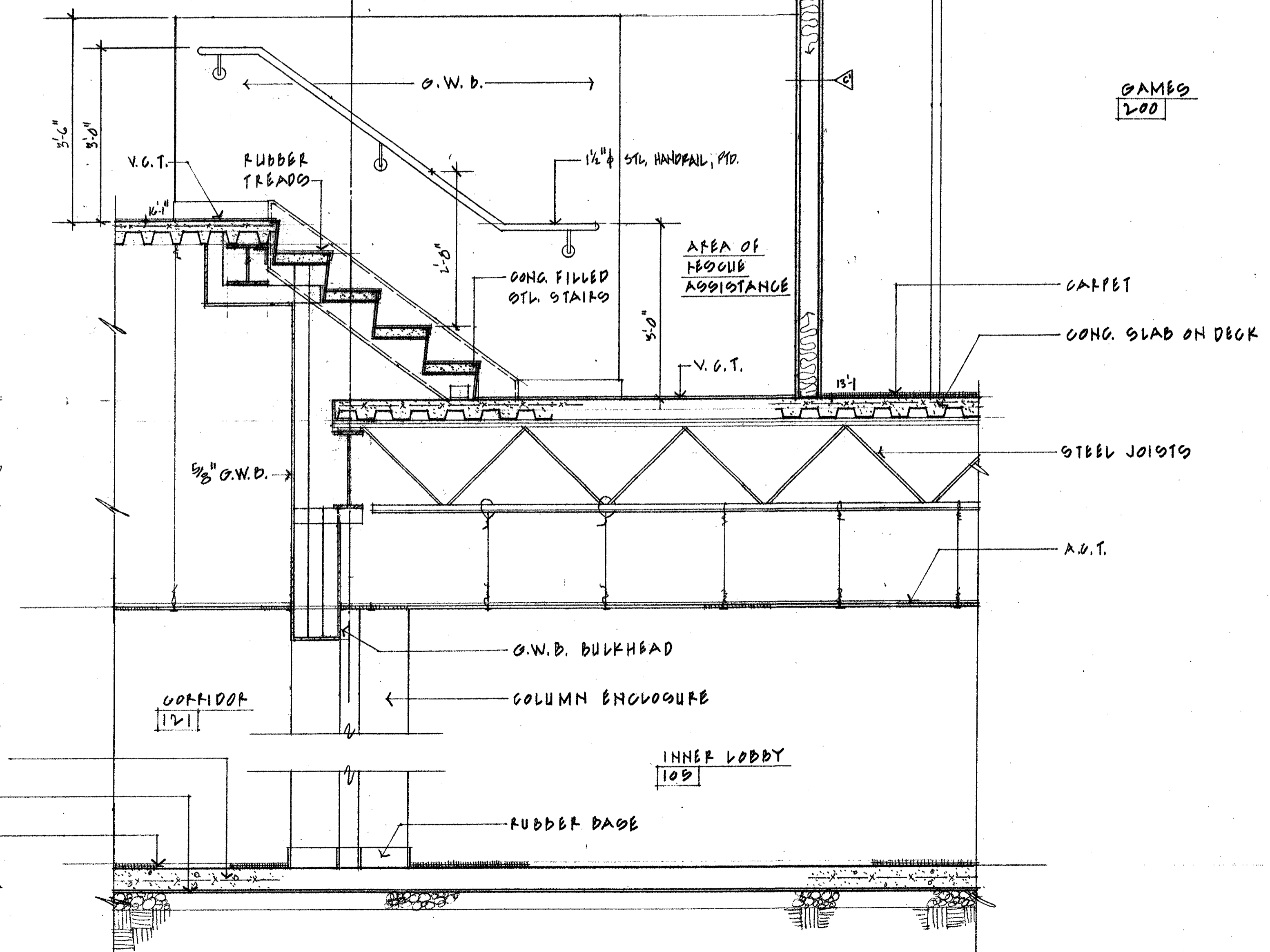
3 WALL SECTION 3/4" = 1'-0"
